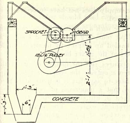
FIG. 21—SIDE ELEVATION BELT CONVEYOR
